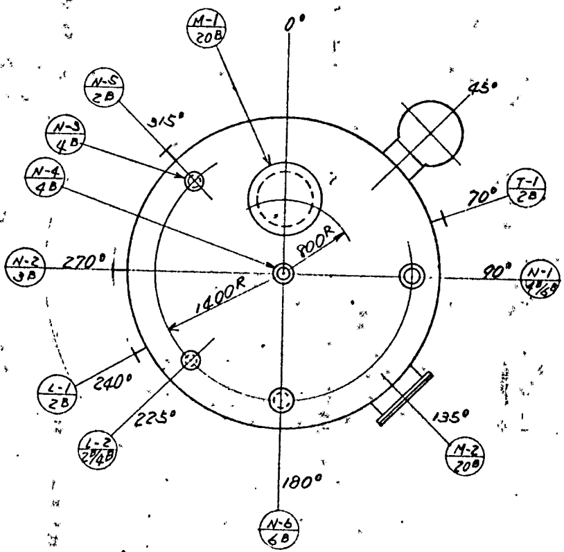
NOZZLE ORIENTATION
