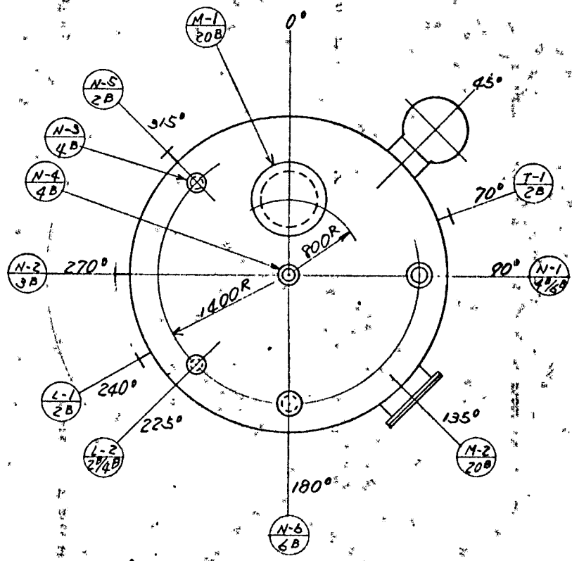
NOZZLE ORIENTATION
