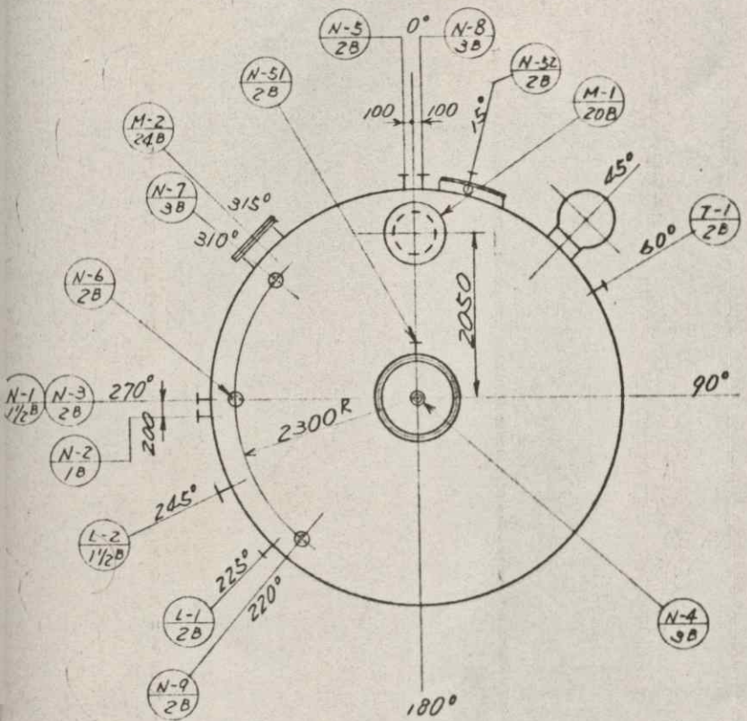
NOZZLE ORIENTATION
